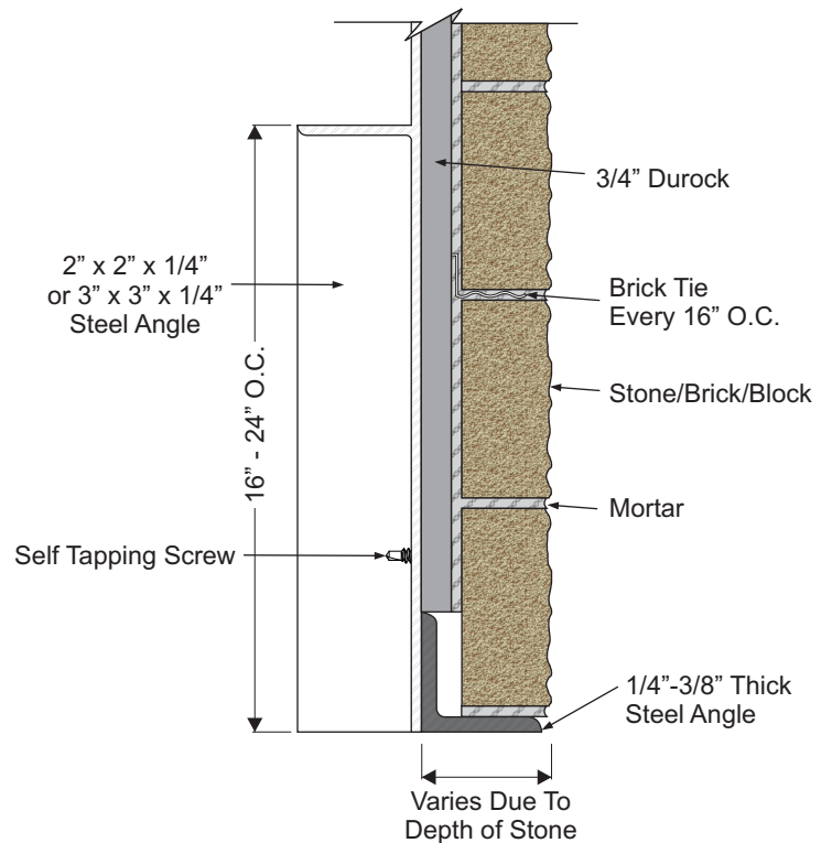
Typical Cross Section ~ Not To Scale
